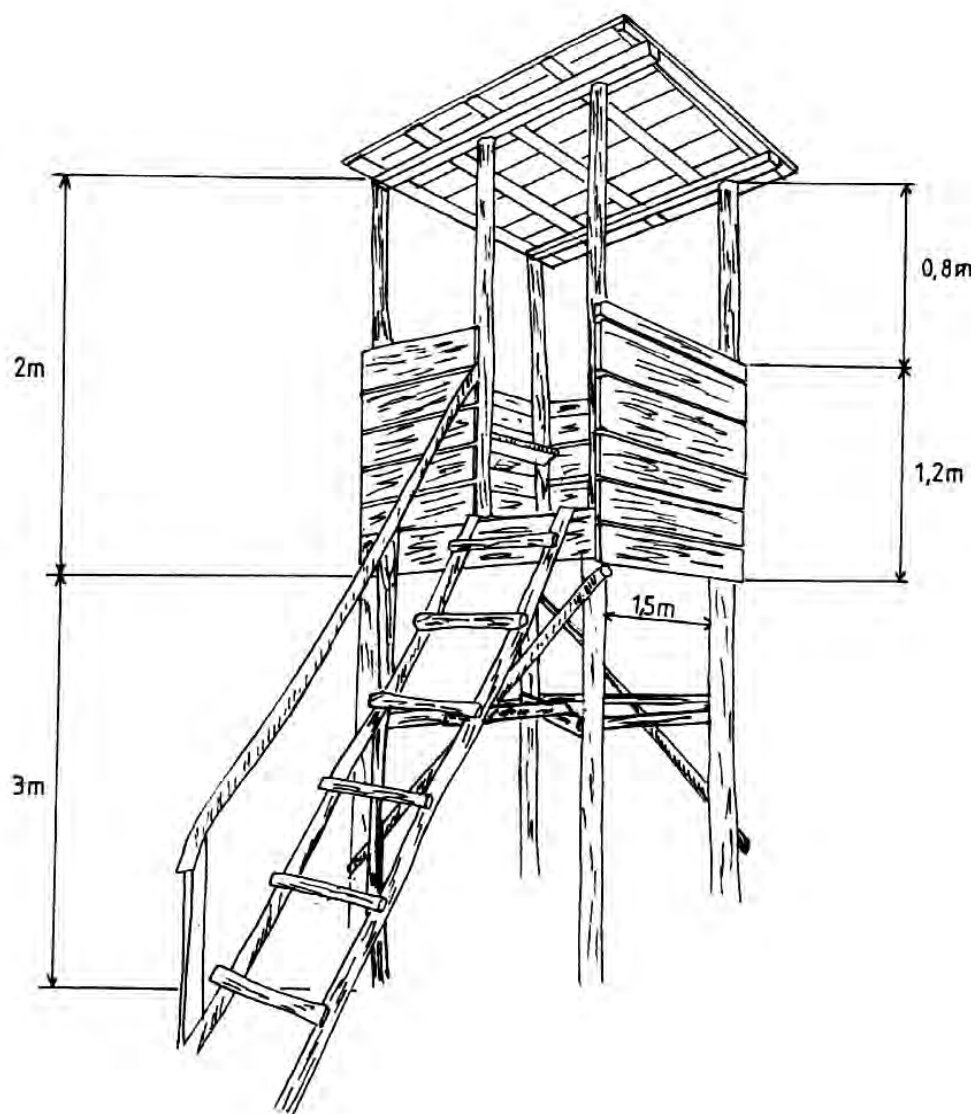
Schia 9. Observator deschis
